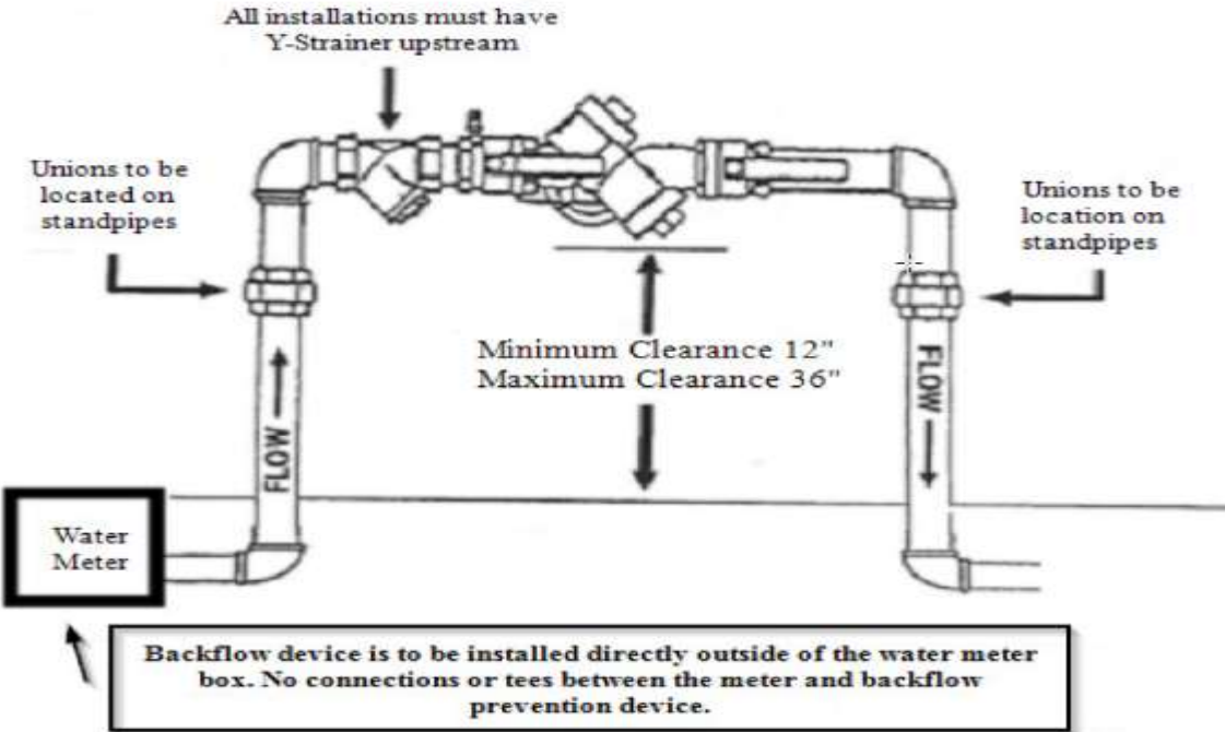
Diagram of Backflow Device
